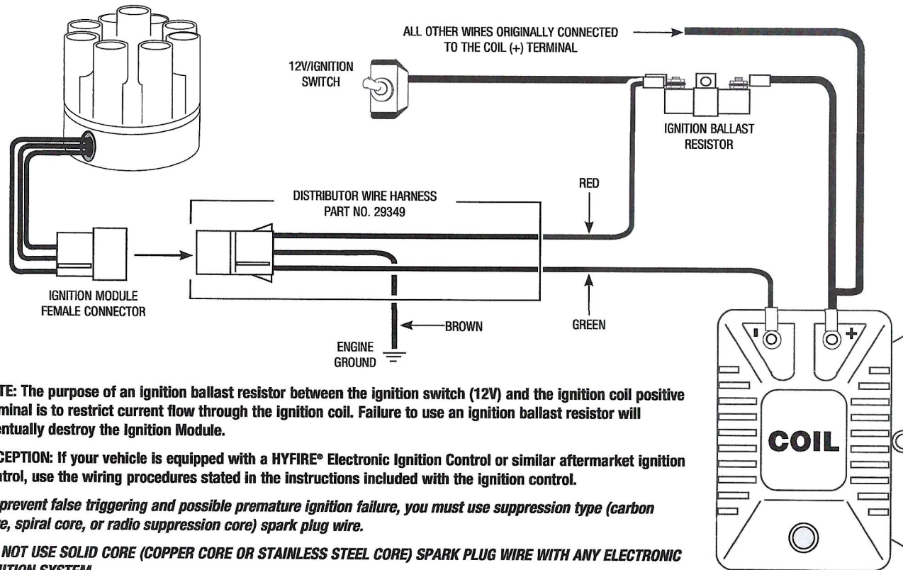
FIGURE 1 UNILITE® WIRING DIAGRAM USING BALLAST RESISTOR
