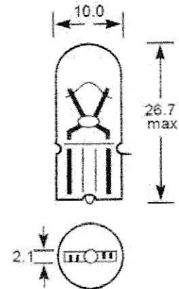
T10 capless wedge base lamp bulb
