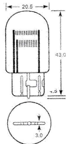
T20 capless wedge base stop/tail lamp bulb
