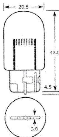
T20 capless wedge base lamp bulb
