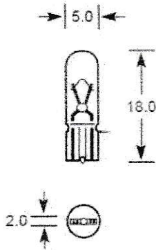
T5 capless wedge base miniature lamp
