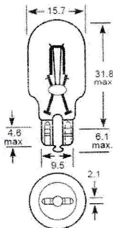
T15 capless wedge base lamp bulb
